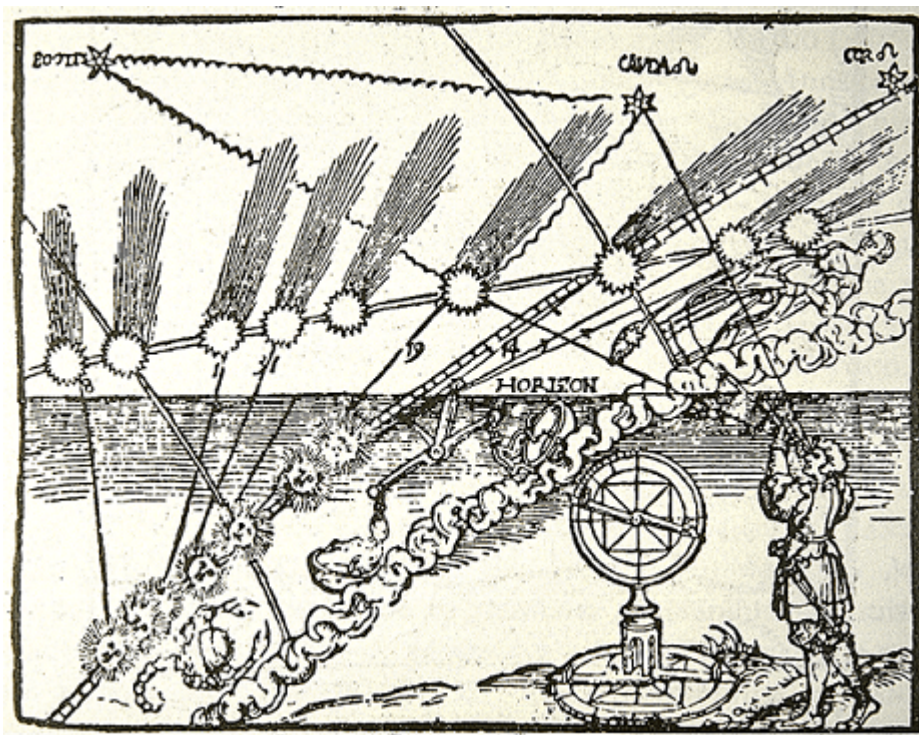
Fig. 3. Observations of comet C/1532 R1 in October and November 1532 by Apian leading to the discovery that cometary tails are directed opposite to the Sun's position in the sky
